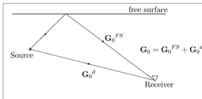
Figure 2. The marine configuration and reference Green's function.
